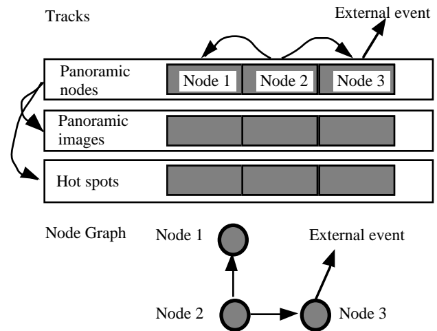
Figure 3. A panoramic movie layout and its corresponding node graph.
