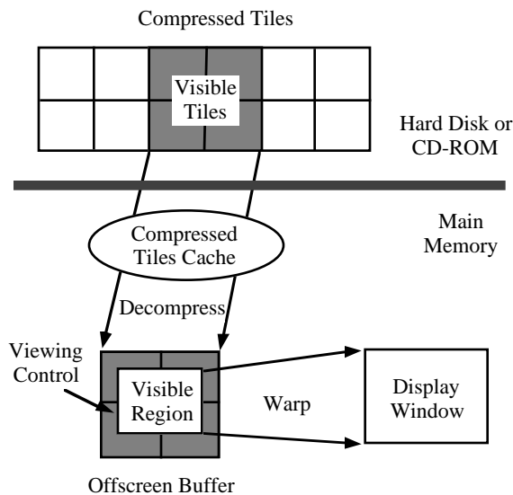
Figure 4. Panoramic display process.
