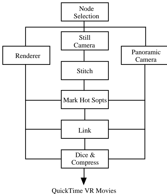
Figure 7. The panoramic movie authoring process.
